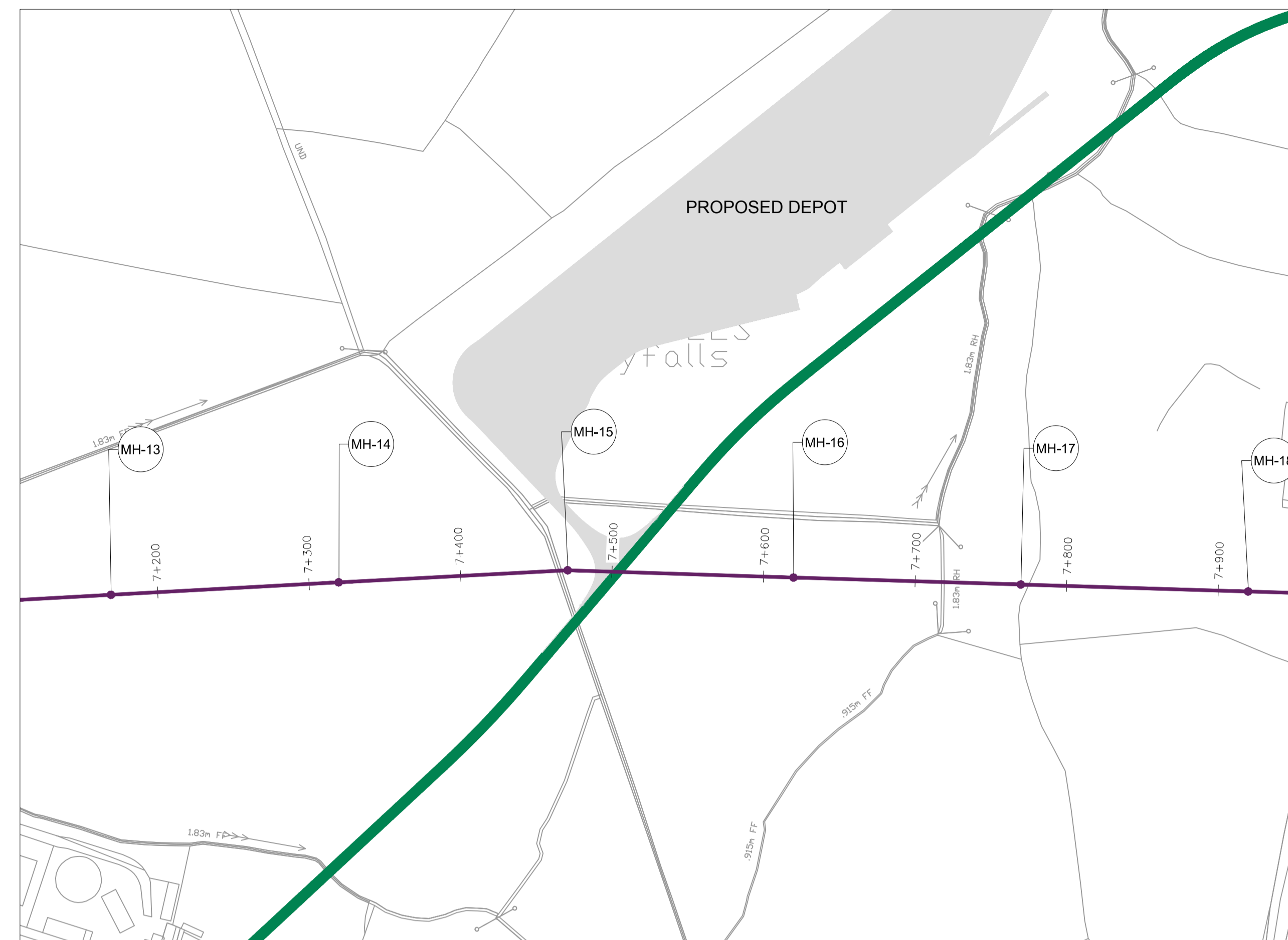
CROSSING POINT 2 (METRO WEST) SCALE: 1:2,500
