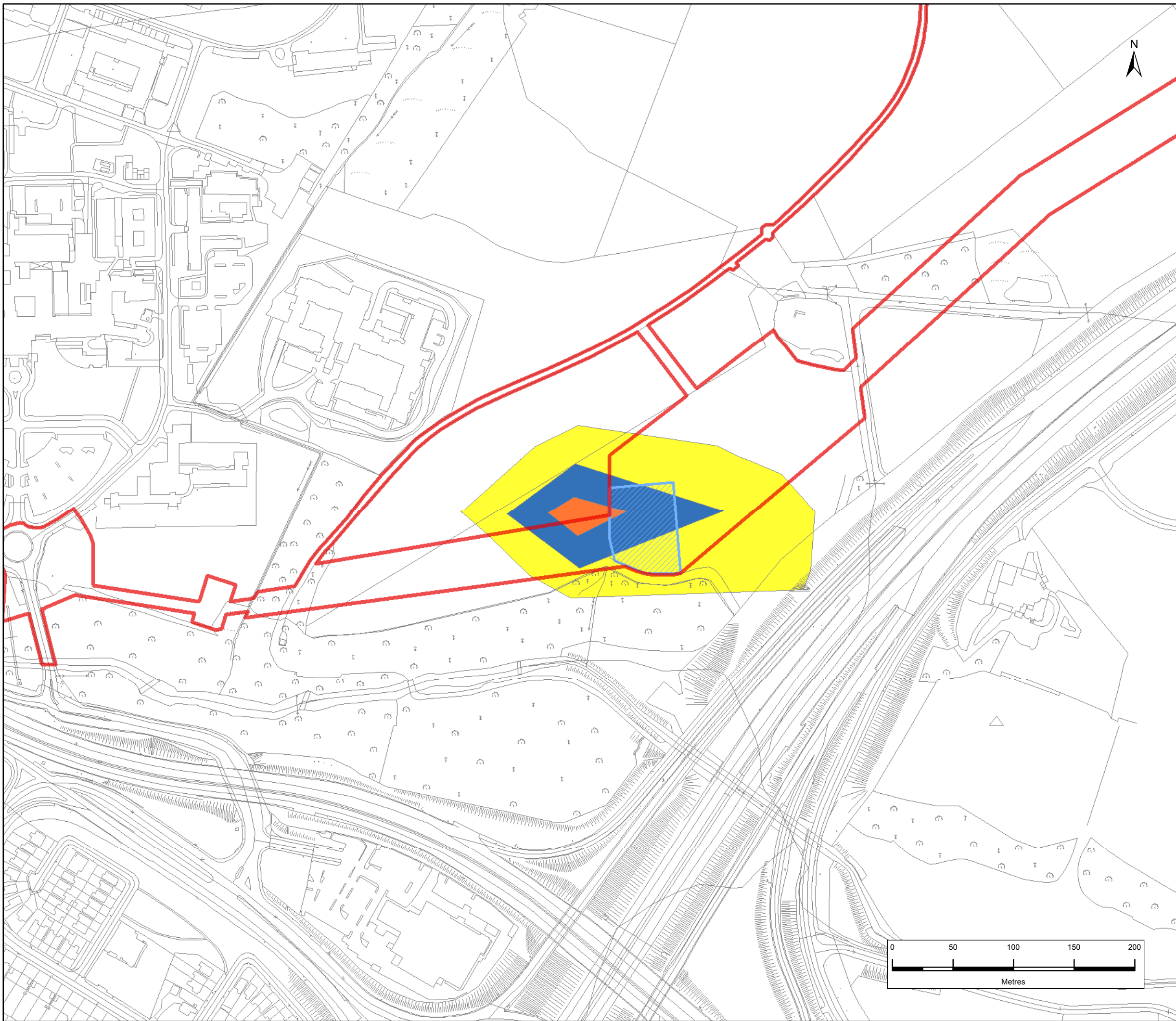
Drawing Title: Figure 14.5 - Isopleth Showing Odour Predictions for 98-percentile of 1-hour Ground Level Odour Concentration for the Proposed Abbotstown Pumping Station for Normal Operating Conditions
